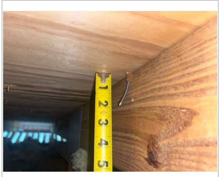
8d Nails
